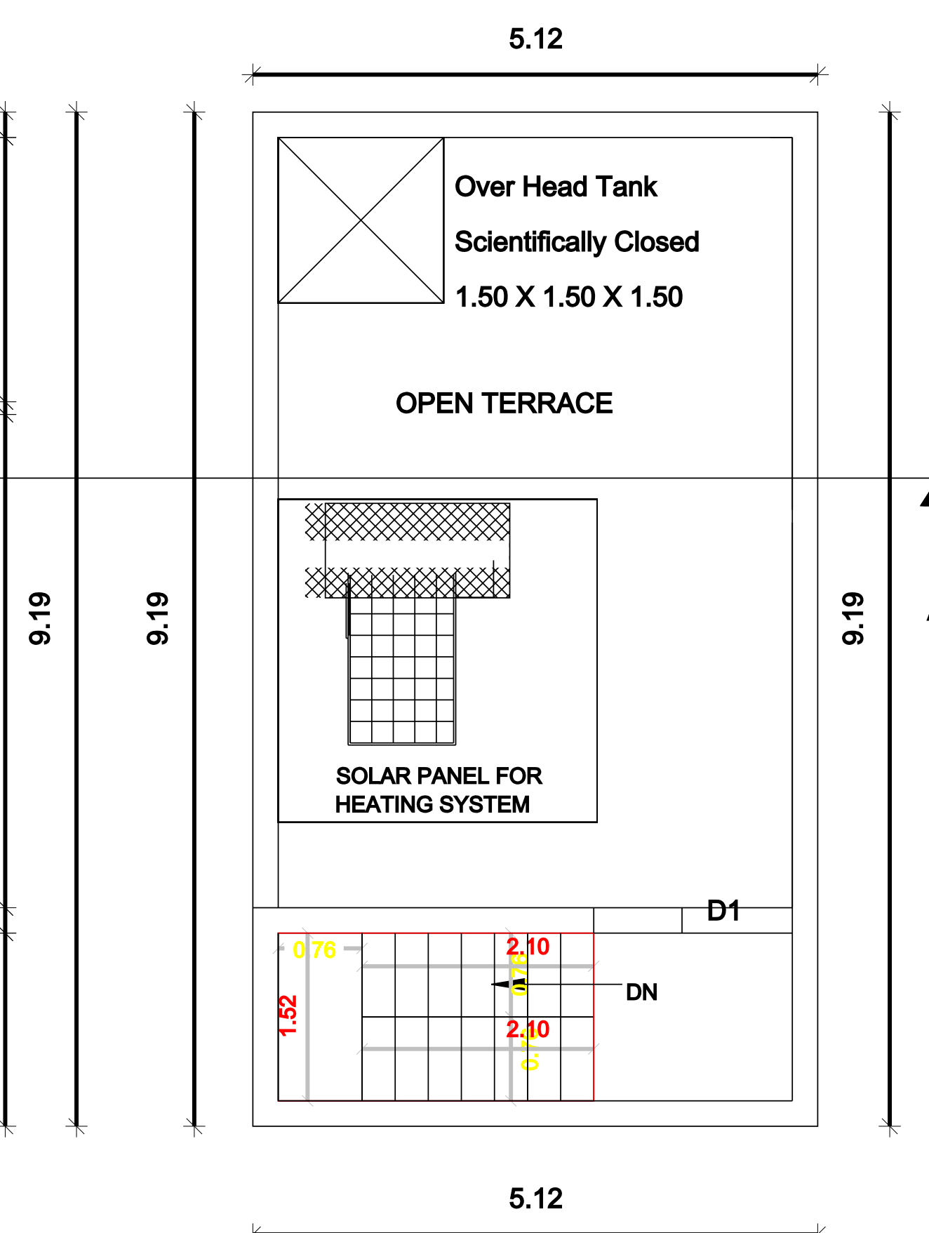
TERRACE FLOOR PLAN PROPOSED
