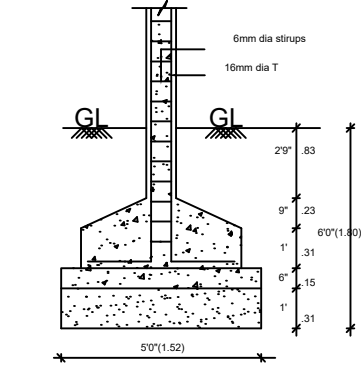
COLUMN FOUNDATION DETAIL SCALE (1:50)
