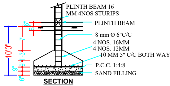
DETAIL OF COLUMN C1,C2
