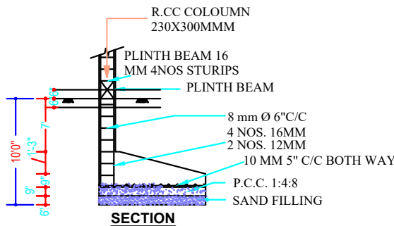
END WALL FOUNDATION
