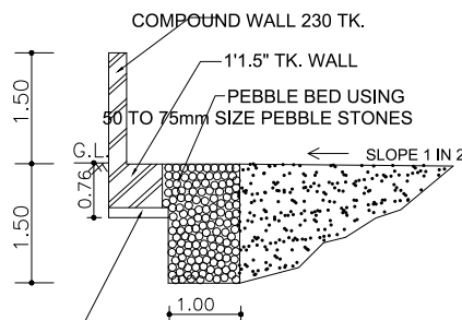
RAIN WATER COLLECTION TRENCH
