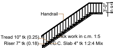
Staircase Details
