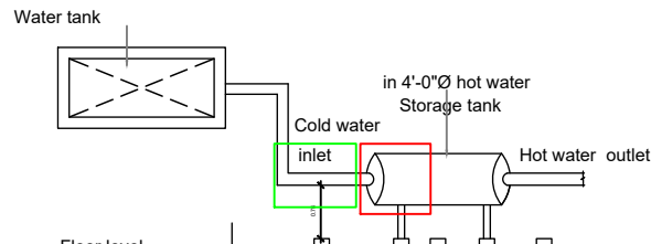
Solar hot water system details
