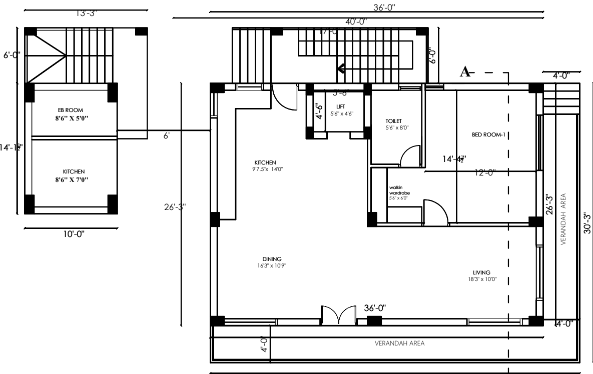
PLAN - GROUND FLOOR
