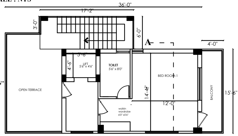
PLAN - SECOND FLOOR
