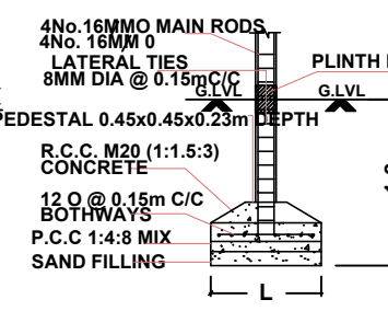
FOUNDATION DETAIL [SCALE: 1:50]
