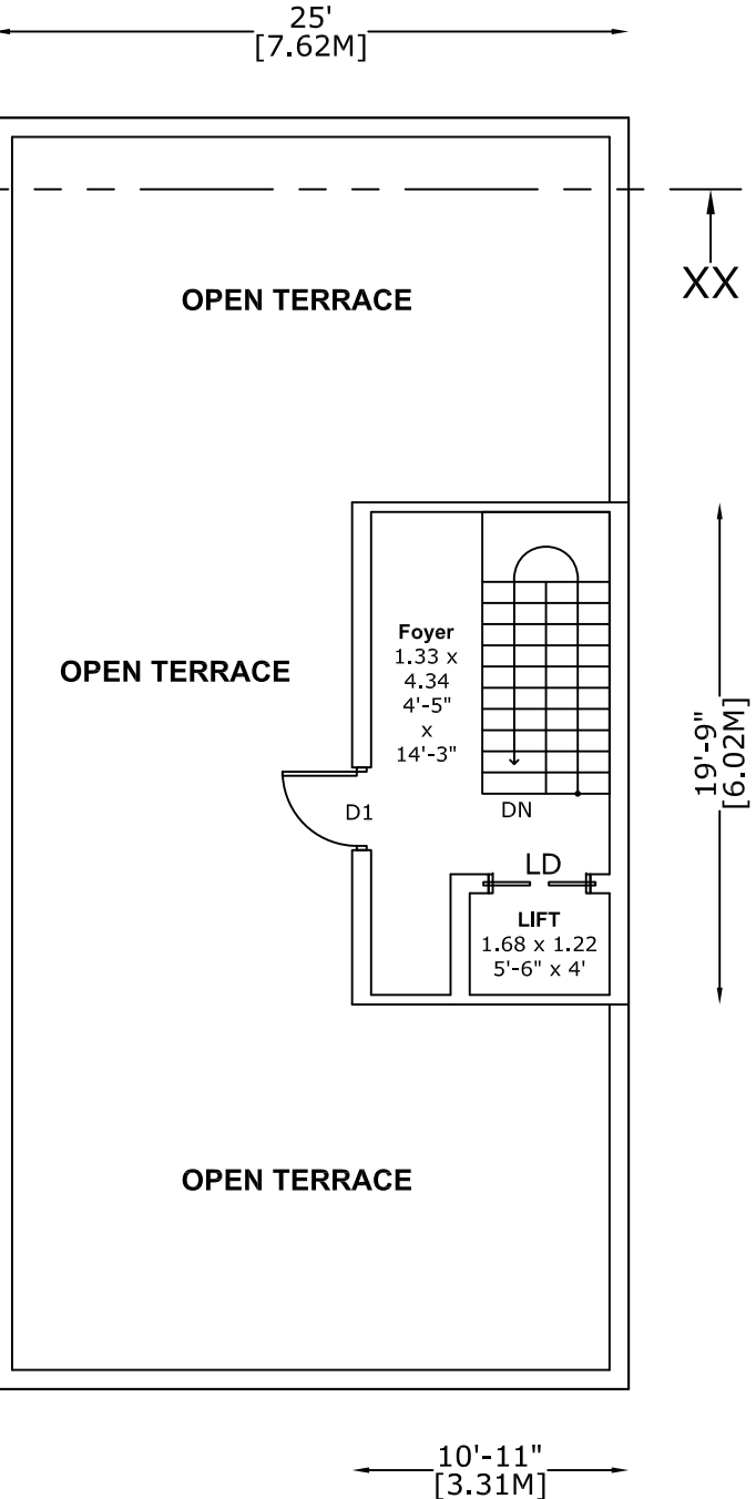
HEAD ROOM / TERRACE FLOOR PLAN
