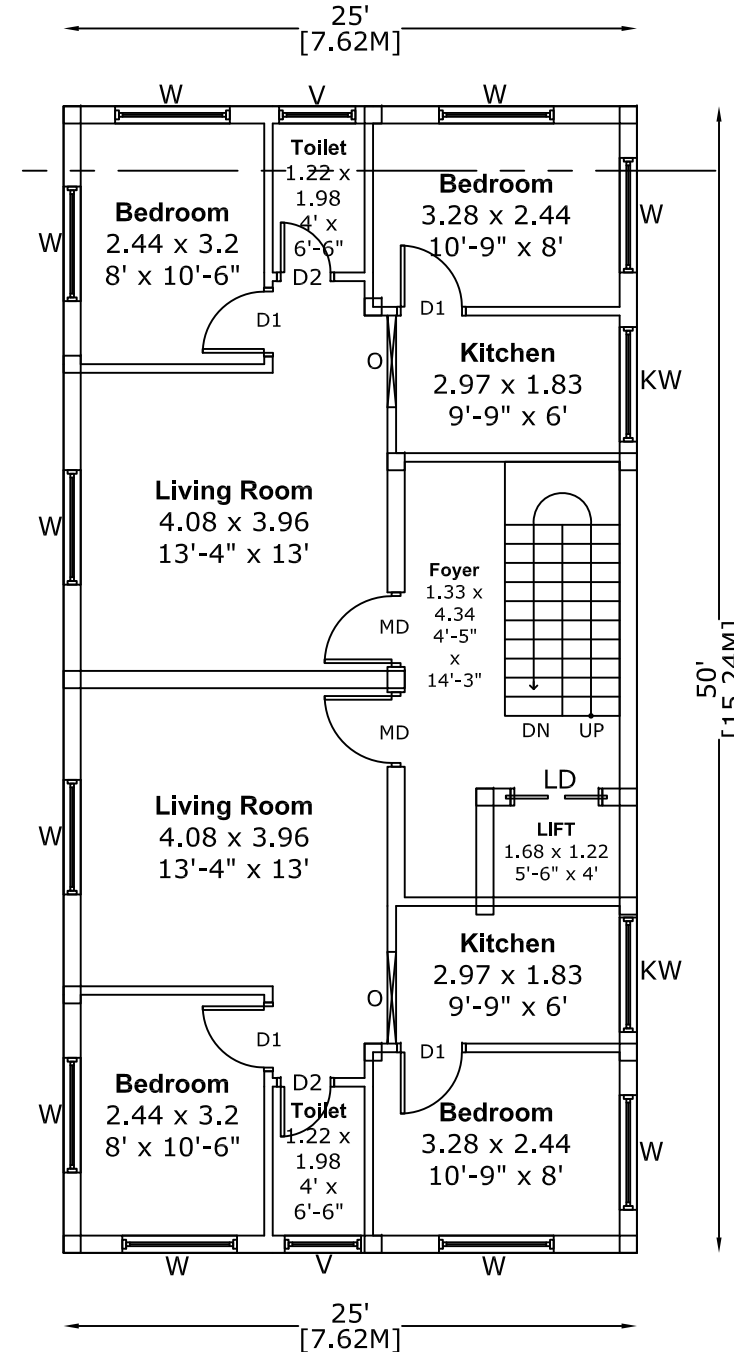
PRO. FIRST FLOOR, SECOND FLOOR & THIRD FLOOR PLAN
