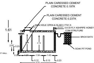
SECTION XX
