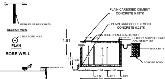
SECTION XX
