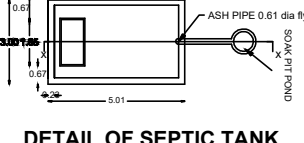
DETAIL OF SEPTIC TANK
