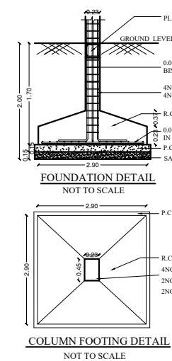
COLUMN FOOTING DETAIL
