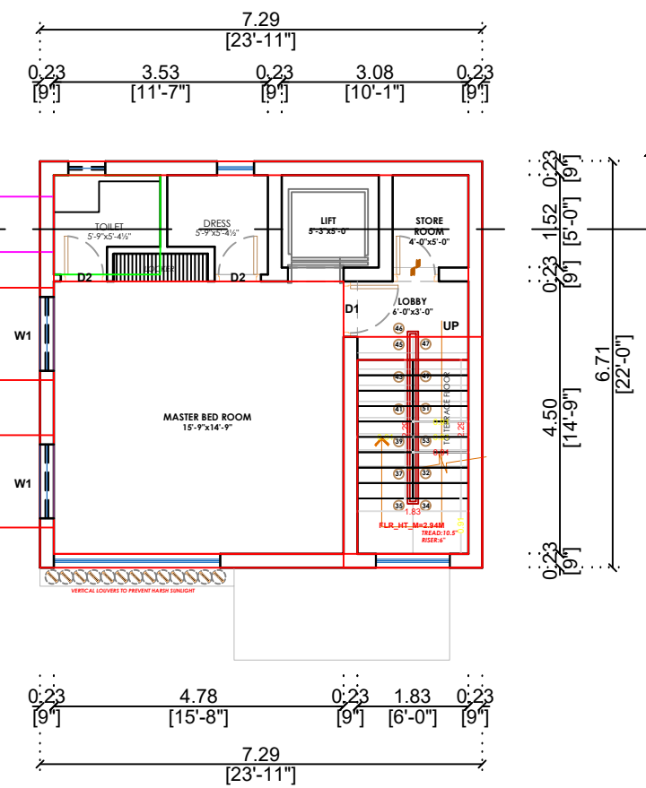
PRO.SECOND FLOOR PLAN
