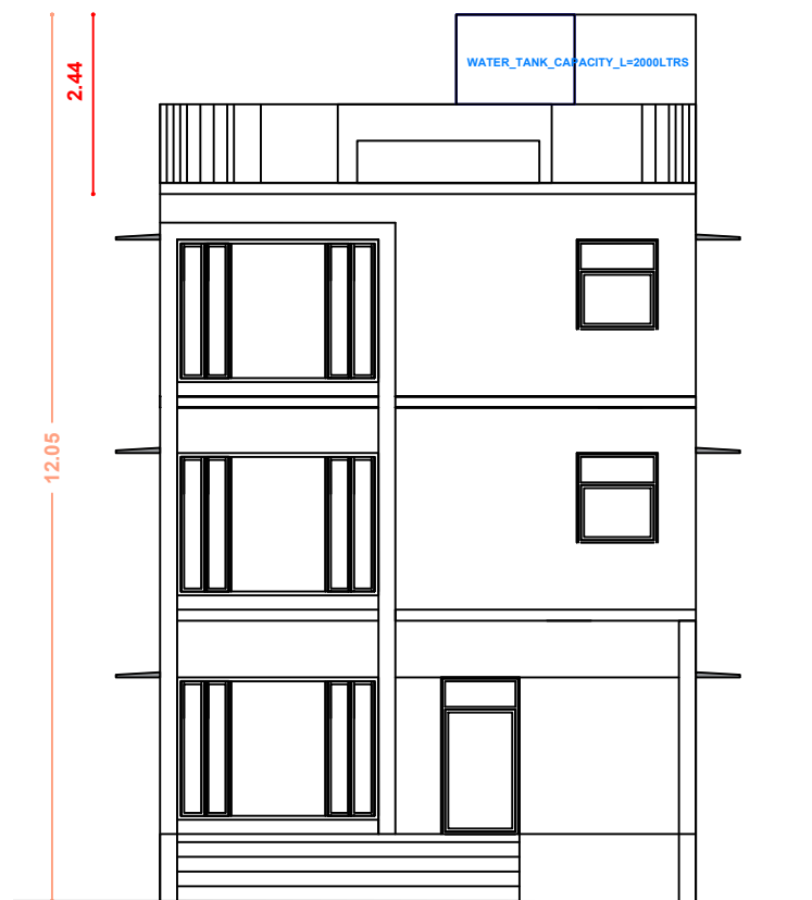
FRONT ELEVATION
