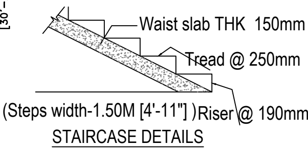
STAIRCASE DETAILS
