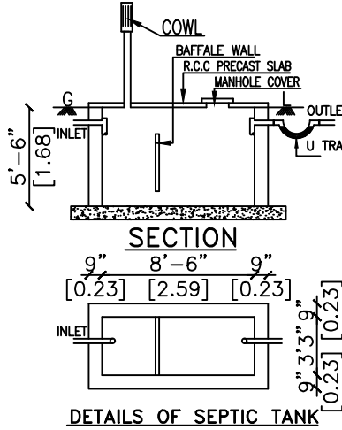
DETAILS OF SEPTIC TANK
