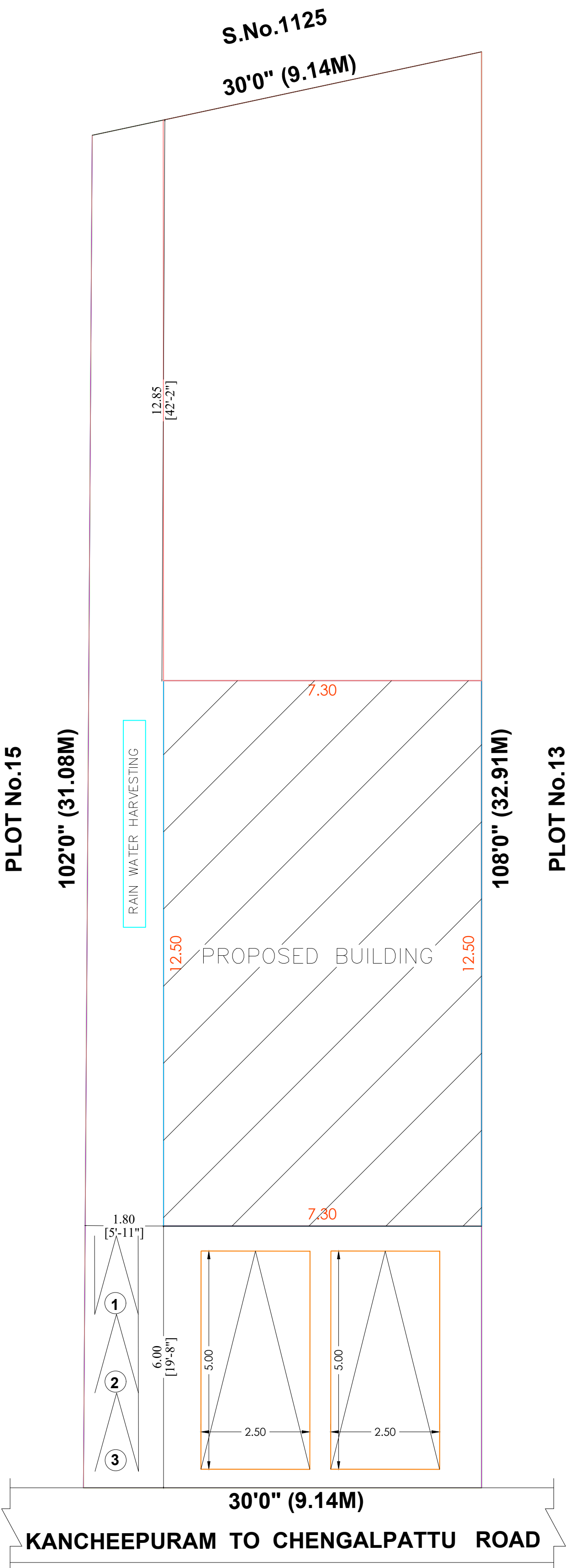
SITE PLAN
