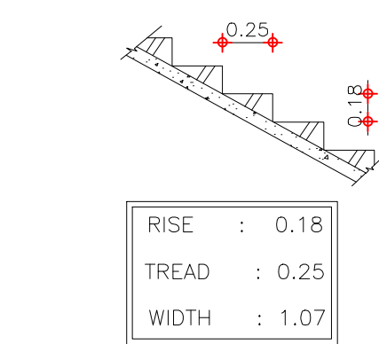
STAIRS DETAILS
