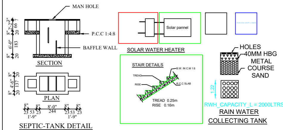
SEPTIC-TANK DETAIL
