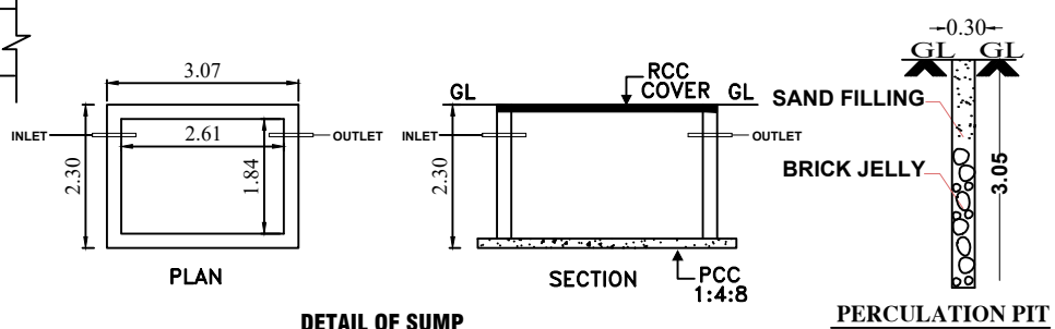
DETAIL OF SUMP
