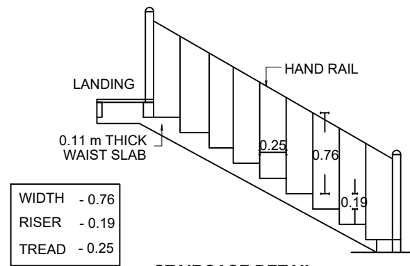
STAIRCASE DETAIL
