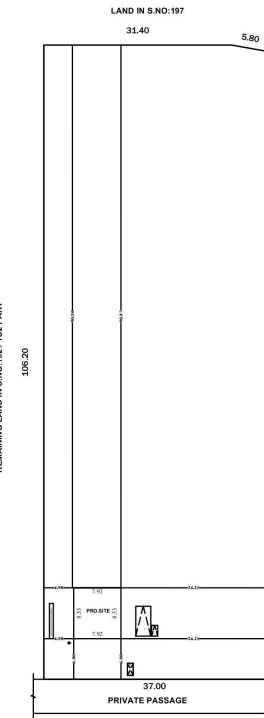
SITE PLAN [1:400]
