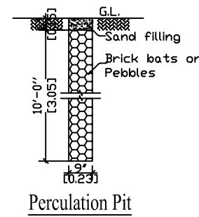
Percolation Pit
