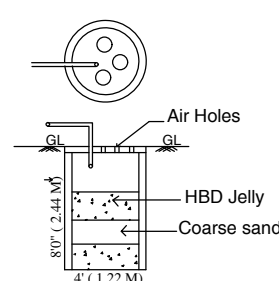
WASTE WATER RECYCLE UNIT
