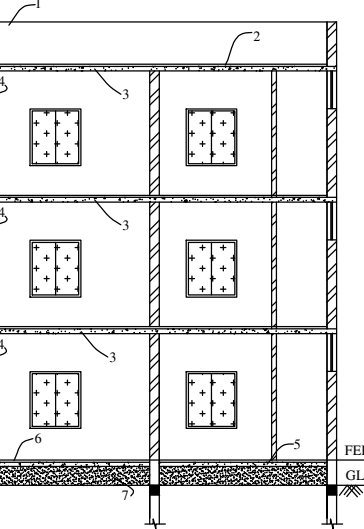
SECTION ON "J-S"
