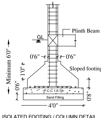
COLUMN DETAILS
