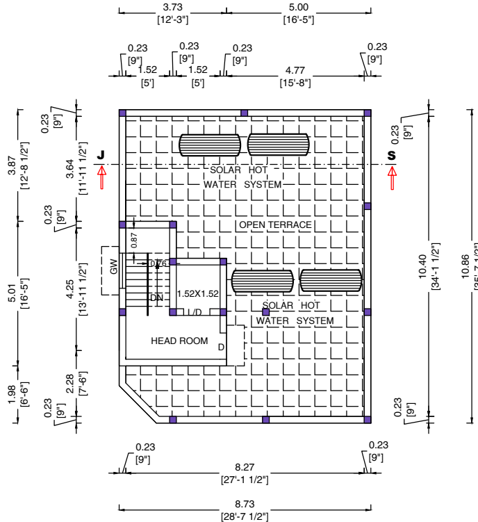
OPEN TERRACE FLOOR PLAN
