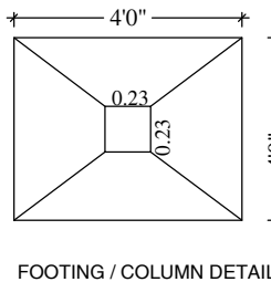
FOOTING / COLUMN DETAIL
