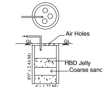
RAIN WATER HARVESTING TANK DETAIL
