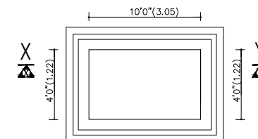
PLAN OF SUMP
