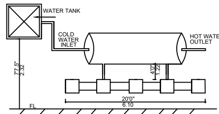
SOLAR HOT WATER SYSTEM DETAILS
