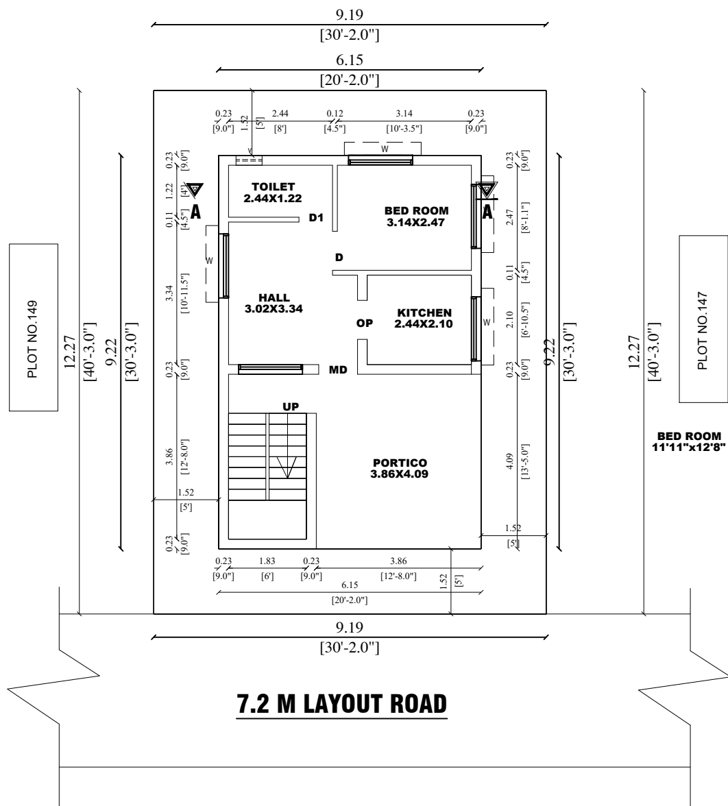
JND FLOOR PLAN
