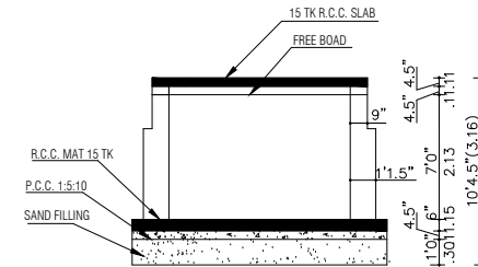
SECTION OF SUMP 'X Y'
