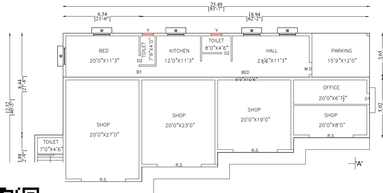
TYPICAL FIRST & SECOND FLOOR PLAN
