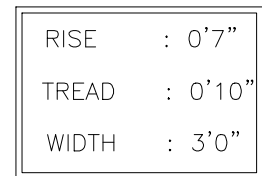
STAIRS DETAILS
