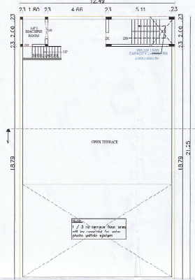
TERRACE FLOOR PLAN (PROPOSED)
