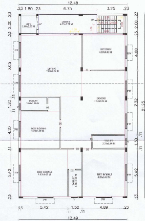
THIRD FLOOR PLAN (PROPOSED)
