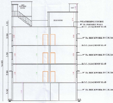
SECTION: V-V
