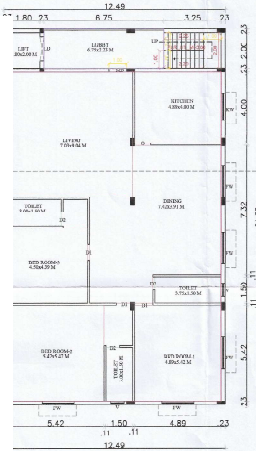
SECOND FLOOR PLAN (PROPOSED)
