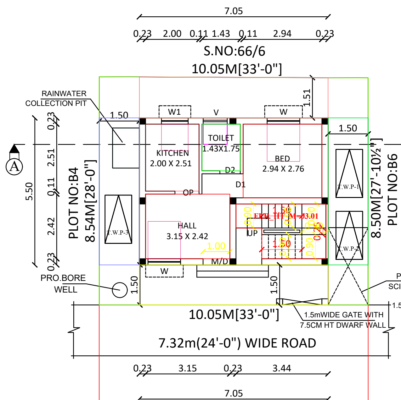
SITE CUM PRO.GROUND FLOOR PLAN
