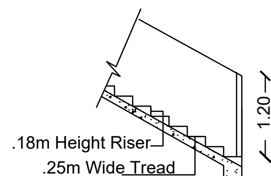
STAIRCASE DETAILS
