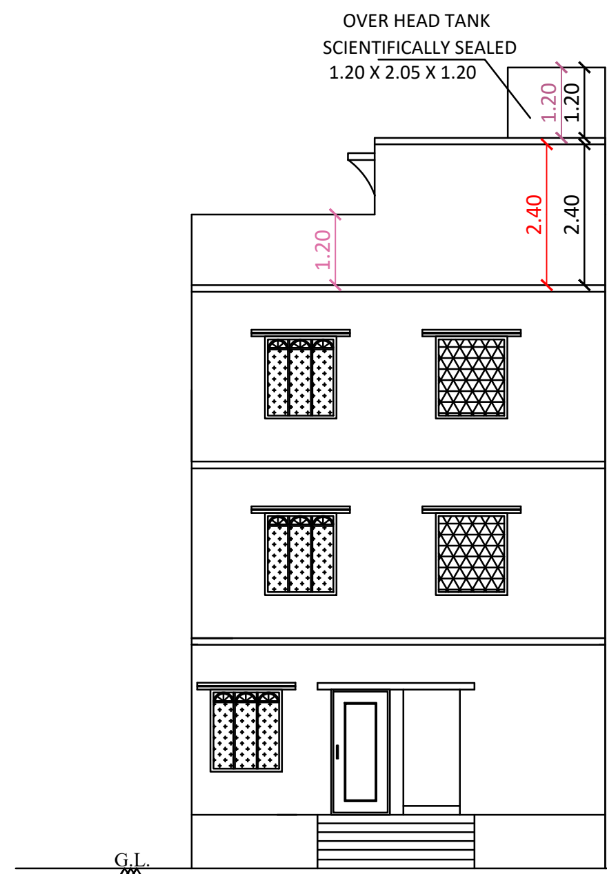
FRONT ELEVATION
