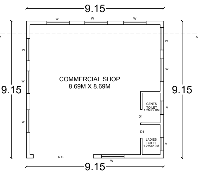
BLOCK -3 PROPOSED COMMERCIAL SHOP BUILDING (RCC BUILDING)
