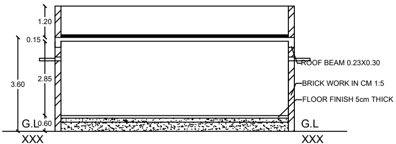
SECTION ON AA BLOCK-3
