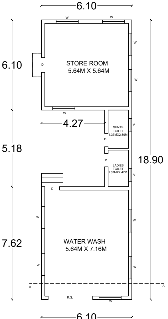
BLOCK -2 PROPOSED COMMERCIAL BUILDING (GALVALUME ROOF BUILDING)
