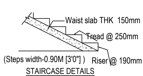
STAIRCASE DETAILS
