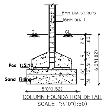
SCALE 1:4'0" (1:50)
