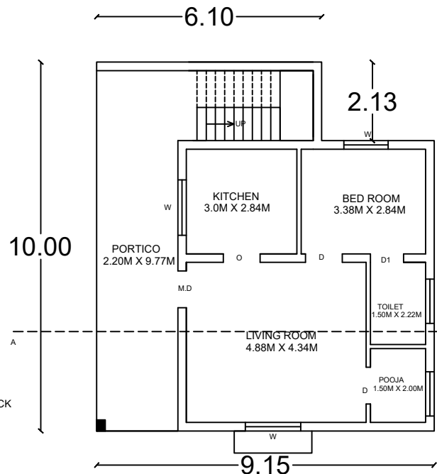
BLOCK -1 PROPOSED RESIDENTIAL GROUND FLOOR BUILDING (RCC BUILDING)
