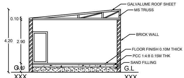
SECTION ON A-A BLOCK-2
