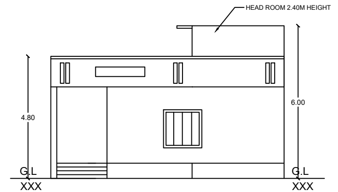
FRONT ELEVATION BLOCK-1
