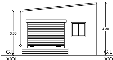
FRONT ELEVATION BLOCK-2
