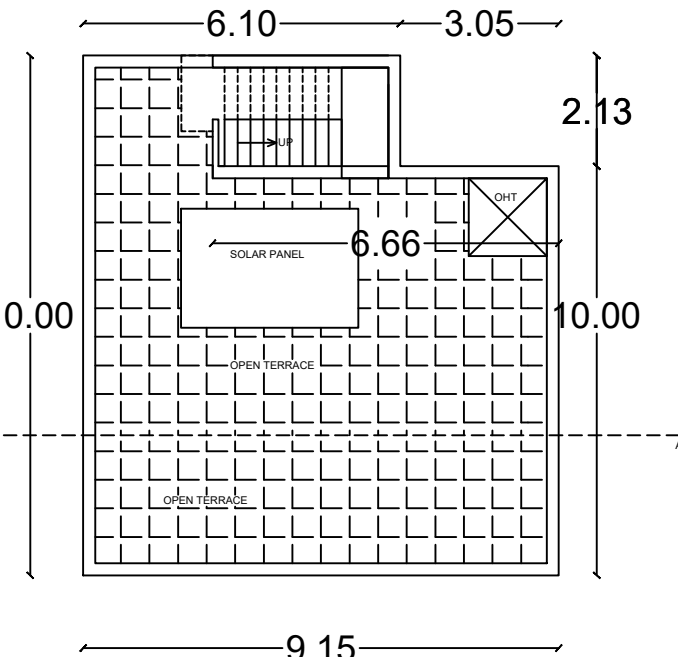
BLOCK -1 PROPOSED RESIDENTIAL TERRACE FLOOR BUILDING
