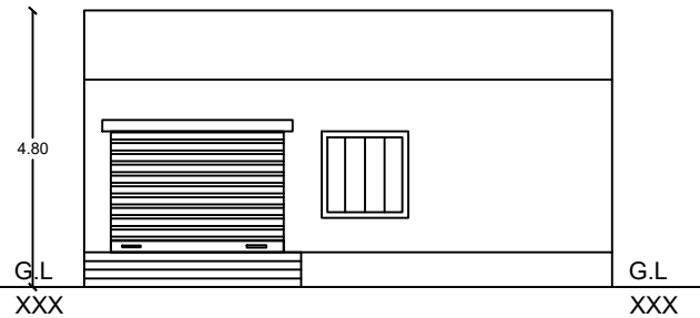
FRONT ELEVATION BLOCK-3
