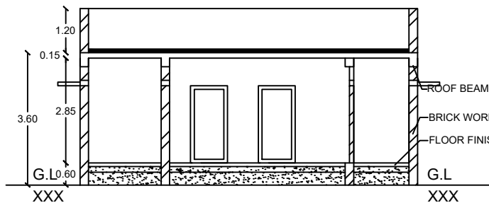
SECTION ON AA BLOCK-1
