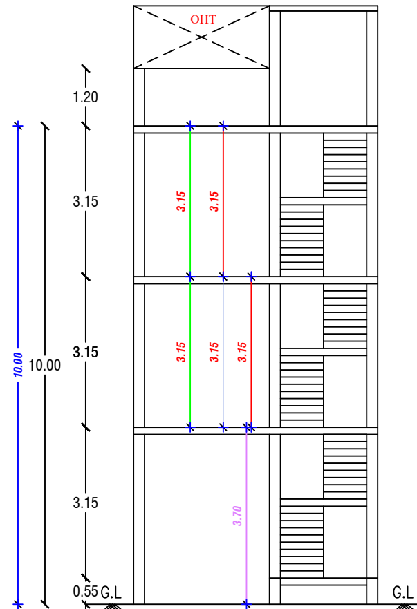
SECTION 'X-X'
