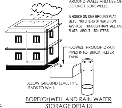
BOREWELL AND RAIN WATER STORAGE DETAILS
