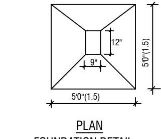
PLAN FOUNDATION DETAIL
