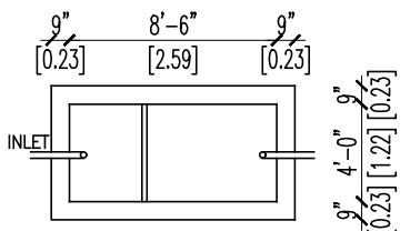
DETAILS OF SEPTIC TANK
