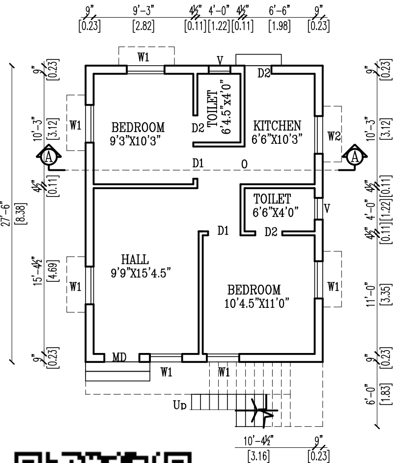
FLOOR PLAN
