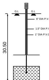
BORE WELL
