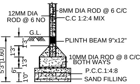
RUN THROUGH COLUMN FOUNDATION SCALE 1"=4'0" (1:50)
