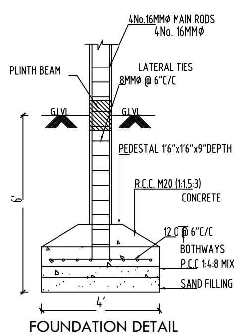
FOUNDATION DETAIL
