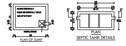
PLAN OF SUMP
