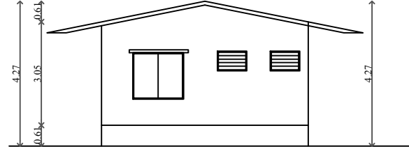
ELEVATION BLOCK -3
