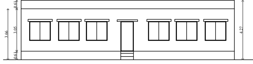
ELEVATION BLOCK -2
