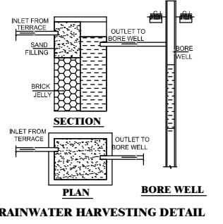
RAINWATER HARVESTING DETAIL
