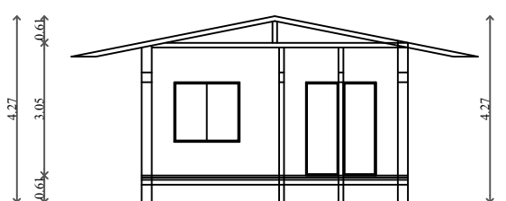
SECTION ON CC BLOCK -3
