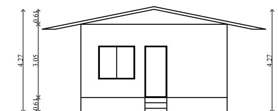
ELEVATION BLOCK -1
