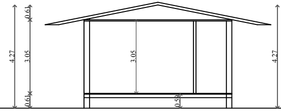
SECTION ON DD BLOCK -1
