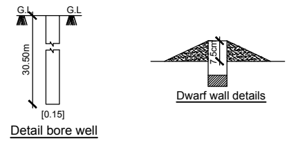
Detail bore well
