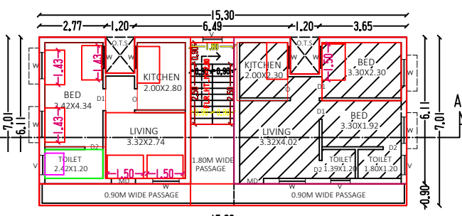
FIRST FLOOR EXISTING AND PROPOSED Scale 1:100
