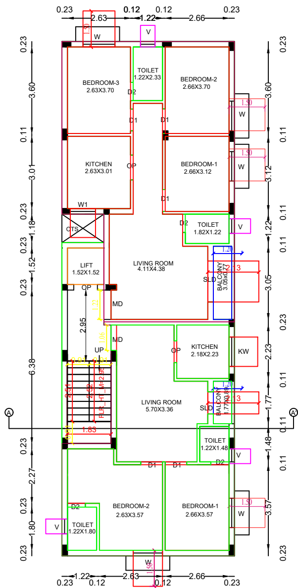
TYPICAL_FLOOR_PLAN=1,2,3 TYPICAL-FIRST, SECOND & THIRD FLOORS PLAN
