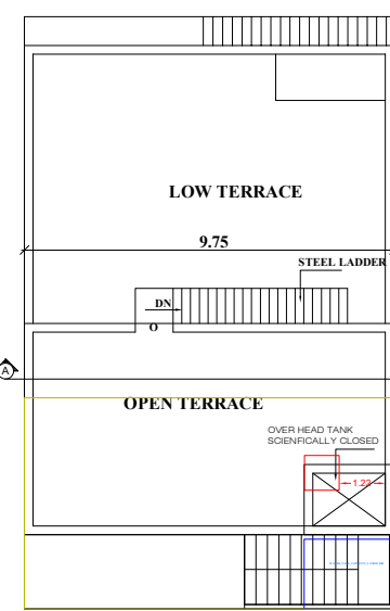
TERRACE FLOOR PLAN (PROPOSED)
