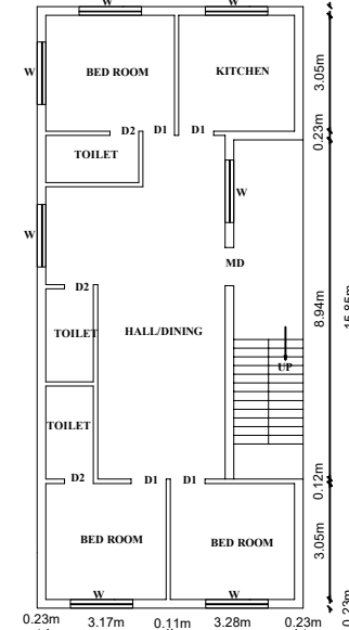
EXISTING GROUND FLOOR PLAN TO BE DEMOLISHED DEMOLITION AREA=111.12 SQ.M
