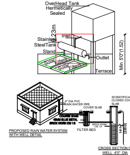
DETAILS OF RAIN WATER HARVEST
