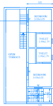
PRO-SECOND FLOOR PLAN
