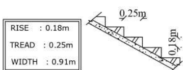
STAIRS DETAILS
