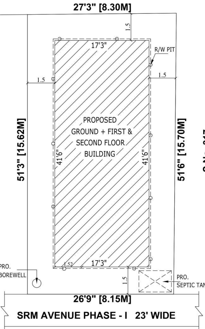
SITE PLAN
