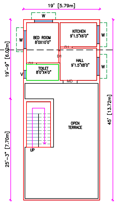
PRO.SECOND FLOOR PLAN
