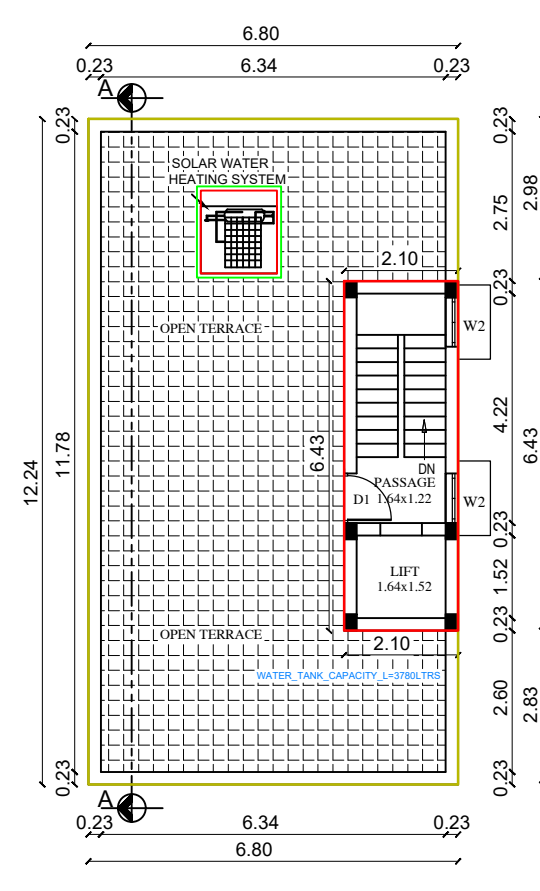
TERRACE FLOOR PLAN (PROPOSED)
