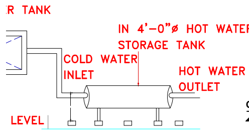
Solar Waterheater Detail
