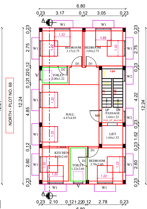
FIRST FLOOR PLAN (PROPOSED)
