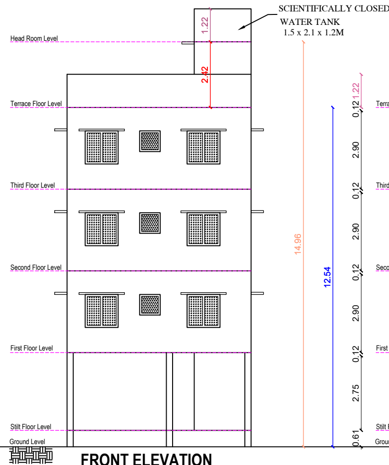
FRONT ELEVATION (PROPOSED)
