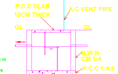
DETAILS OF SEPTIC TANK
