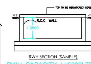
RWH CAPACITY L=5000LTRS
