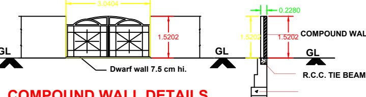
COMPOUND WALL DETAILS
