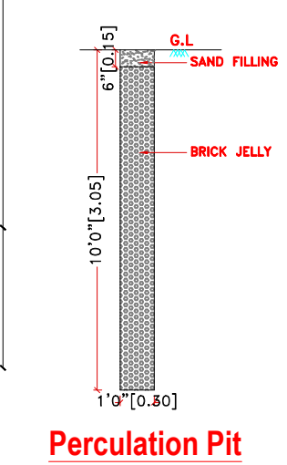
Percolation Pit
