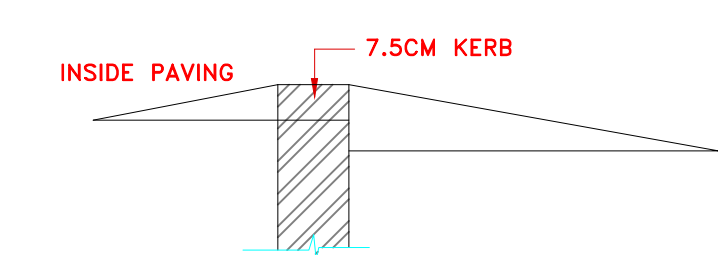
DWARF WALL SECTION
