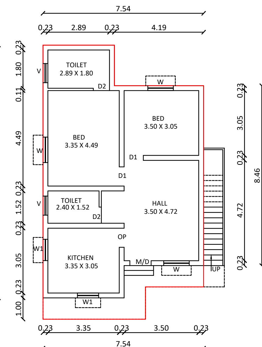
EXG.GROUND FLOOR PLAN Exg. Building to be Demolished AREA:85.04 Sq.Mt(915 Sq.Ft)
