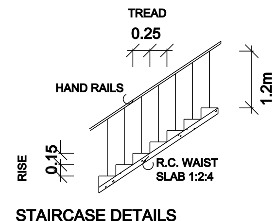
STAIRCASE DETAILS
