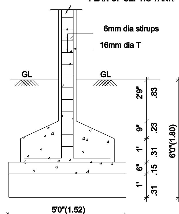
COLUMN FOUNDATION DETAIL
