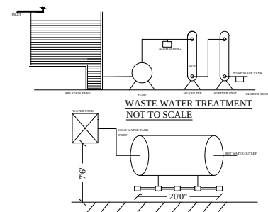
SOLOR HOT WATER SYSTEM DETAILS
