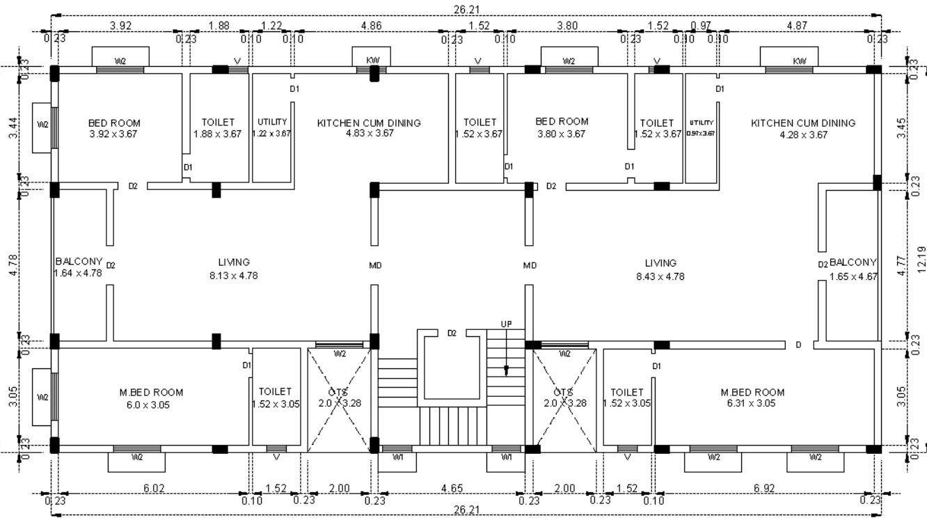
TYPICAL FIRST & SECOND FLOOR PLAN
