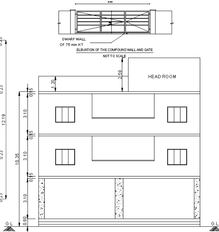
FRONT ELEVATION
