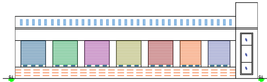
FRONT ELEVATION
