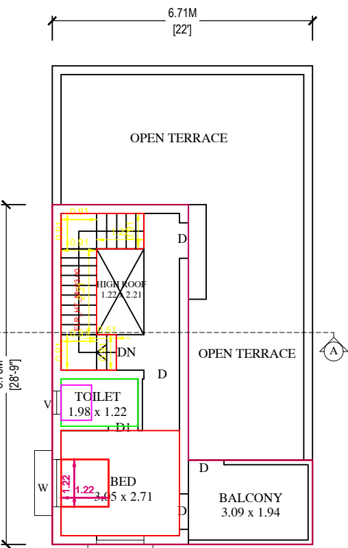
PRO.SECOND FLOOR
