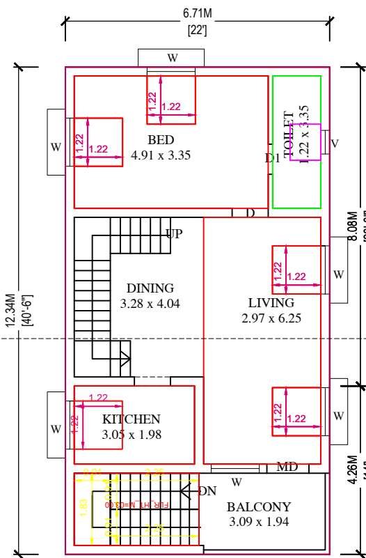
PRO.FIRST FLOOR
