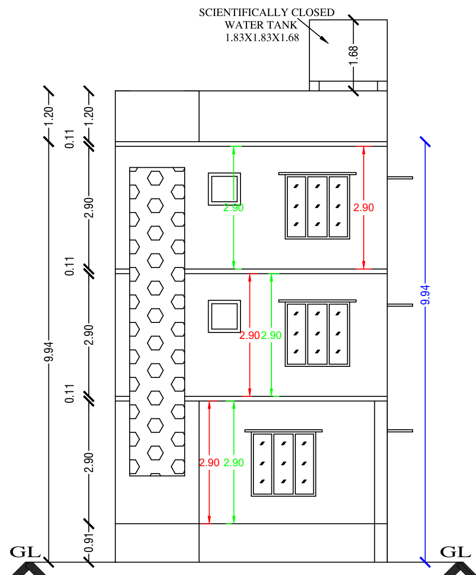
FRONT ELEVATION
