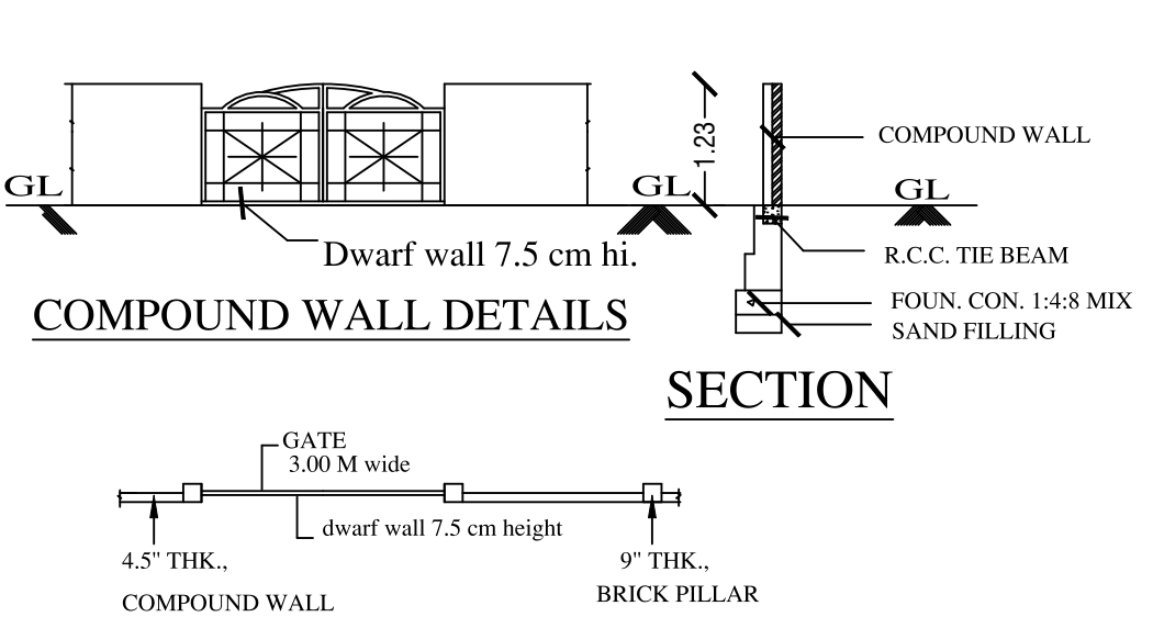
COMPOUND WALL PLAN
