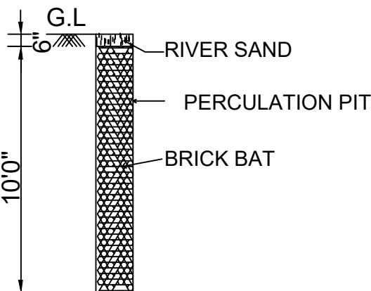
PERCOLATION PIT
