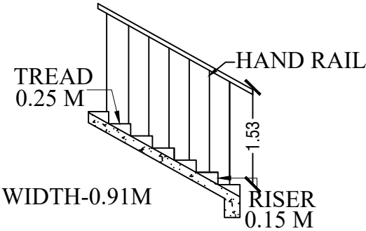
STAIRCASE DETAILS
