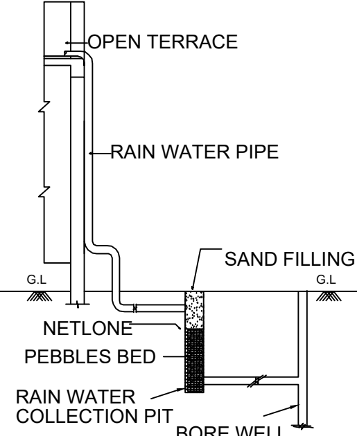
RAIN WATER
