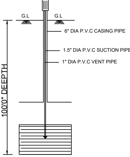
BORE WELL
