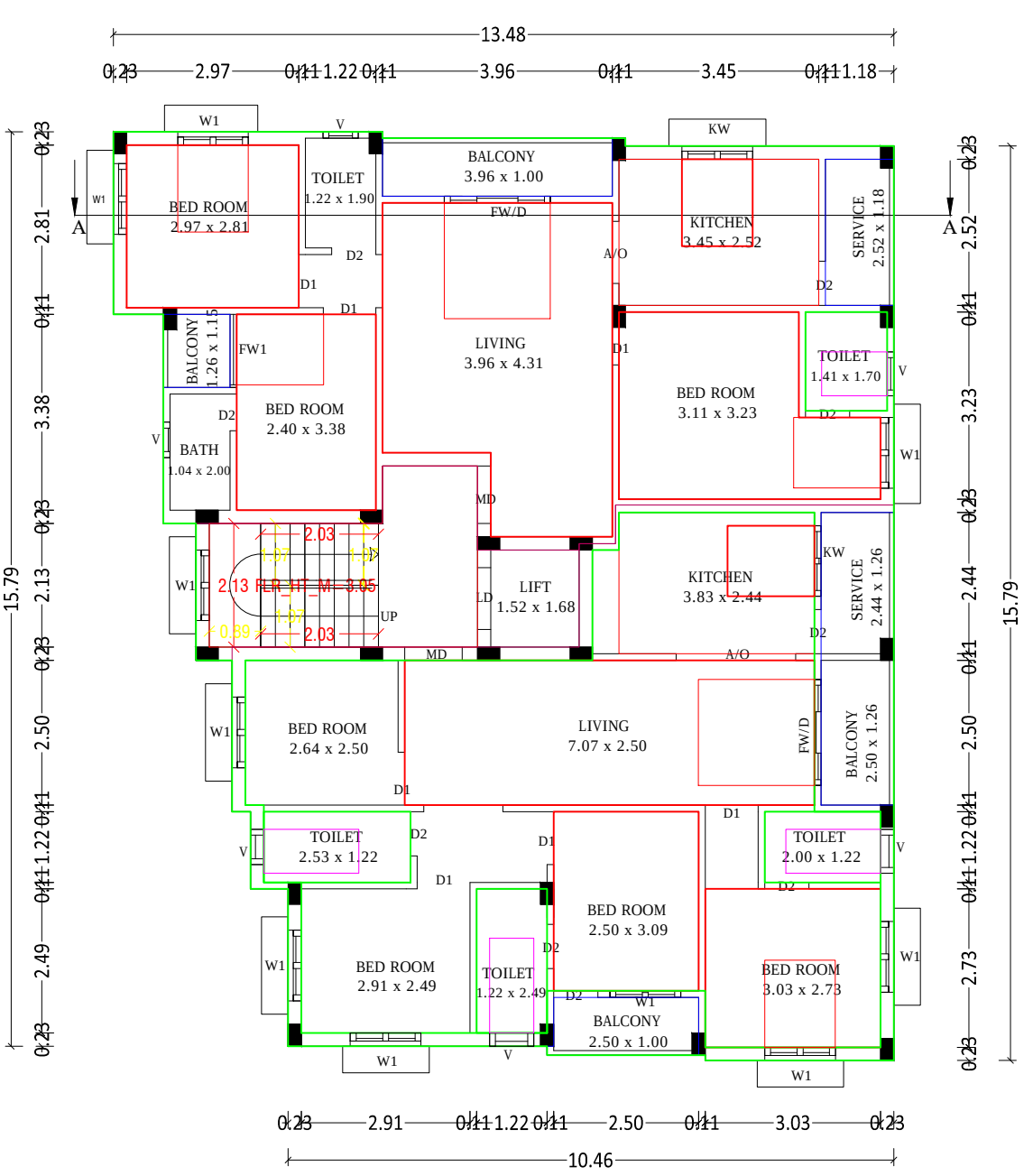
TYPICAL FLOOR PLAN=1,2,3 ( PROPOSED )
