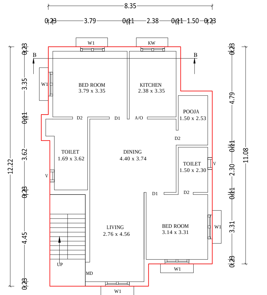
FIRST FLOOR PLAN ( TO BE DEMOLISHED )
