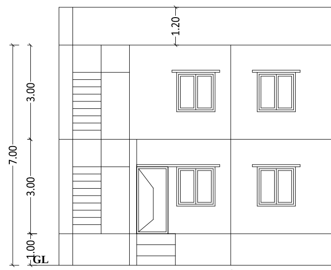
ELEVATION ( TO BE DEMOLISHED )
