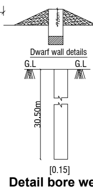
Detail bore well
