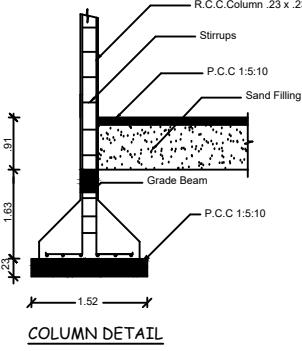
COLUMN DETAIL
