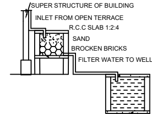
RAINWATER HARVESTING
