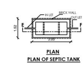
PLAN OF SEPTIC TANK
