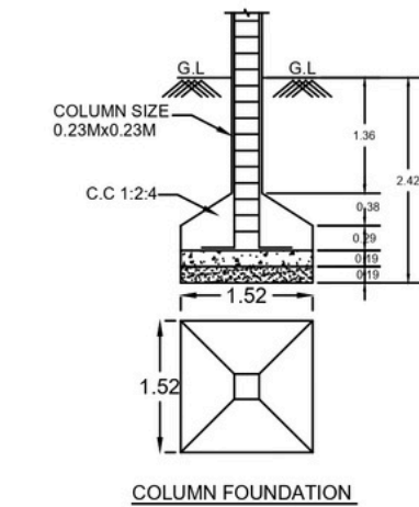
COLUMN FOUNDATION
