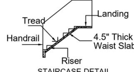
STAIRCASE DETAIL
