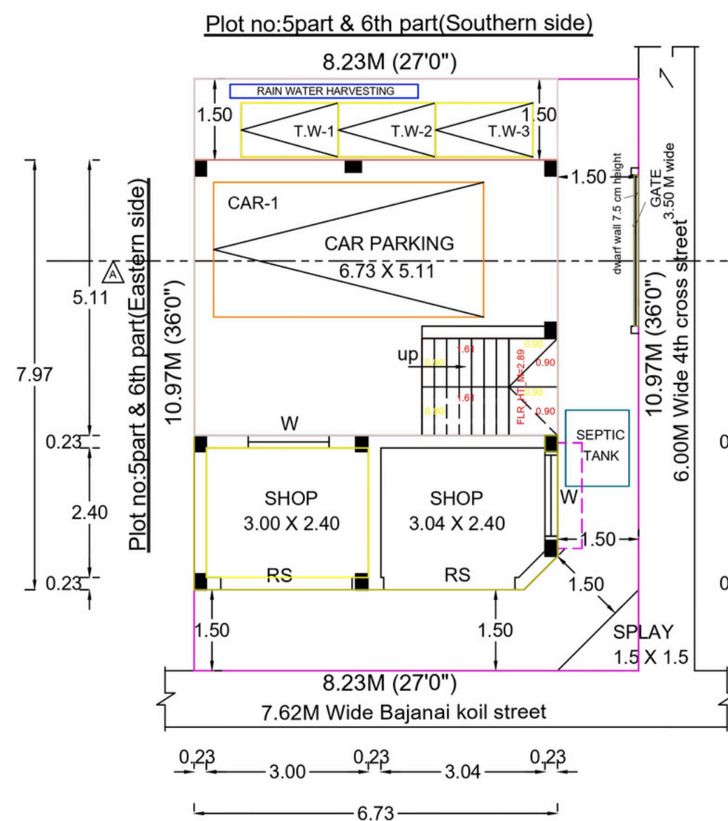
SITE CUM GROUND FLOOR PLAN
