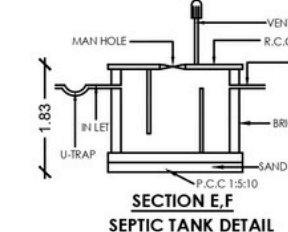
SECTION E.F. SEPTIC TANK DETAIL
