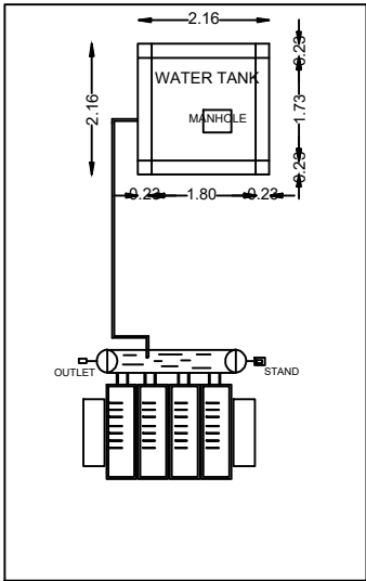
PLAN OF OHT SOLAR WATER HEATING SYSTEM
