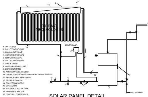
SOLAR PANEL DETAIL
