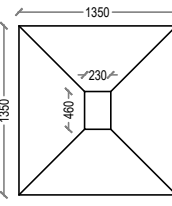
FOUNDATION DETAIL
