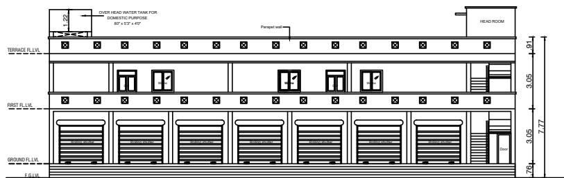
FRONT ELEVATION (PROPOSED)
