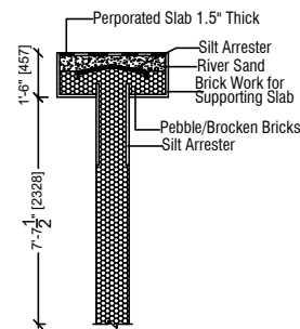
PERCOLATION PIT
