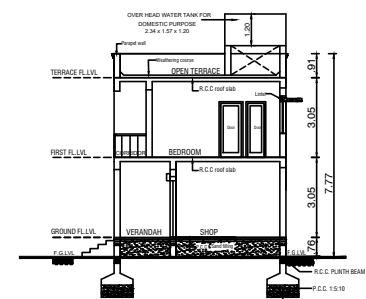
SECTION - AA' (PROPOSED)
