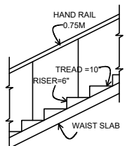
DETAILS OF STAIRCASE (SCALE= 1": 4'0")
