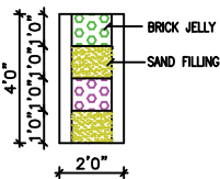
PERCOLATION PIT
