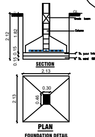
FOUNDATION DETAIL
