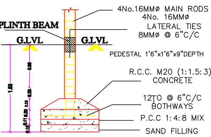
Foundation Detail [Scale: 1:50]
