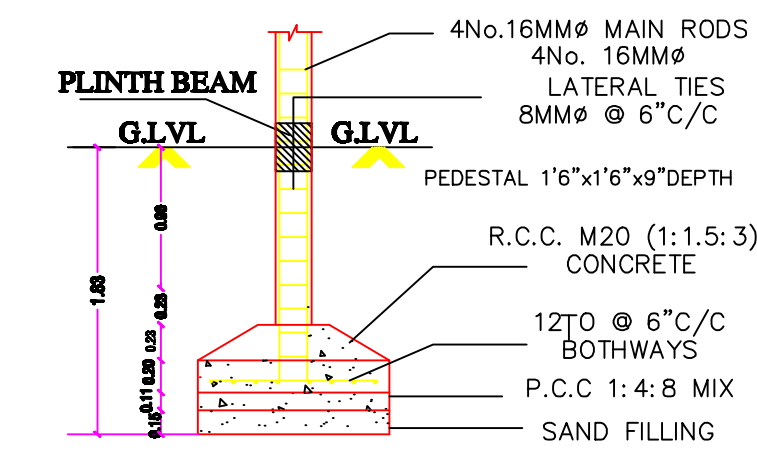
Foundation Detail [Scale: 1:50]
