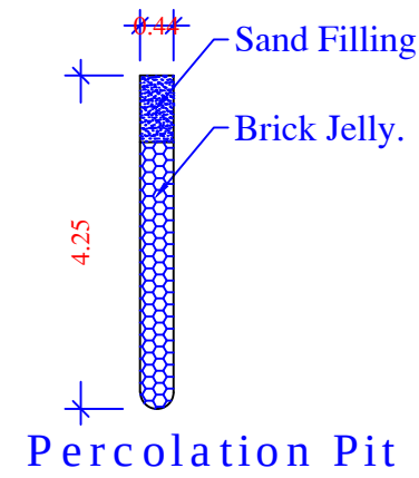
Percolation Pit
