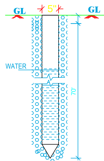
BORE WELL DETAIL PROPOSED
