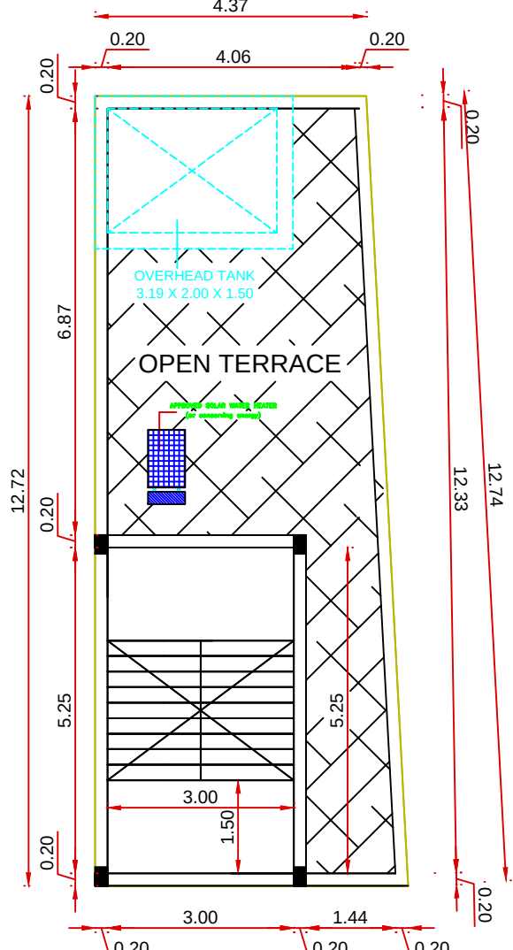
TERRACE FLOOR PLAN (PROPOSED)
