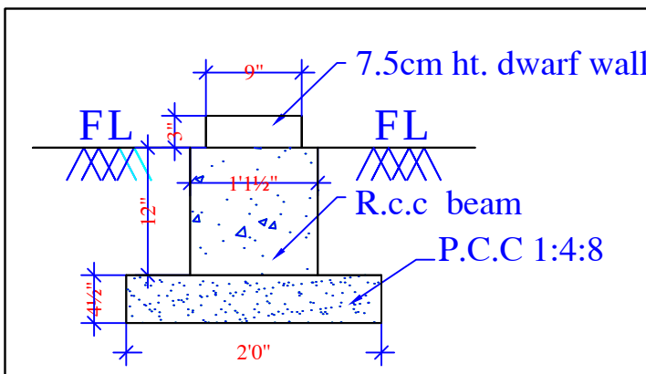
Dwarf Wall Section
