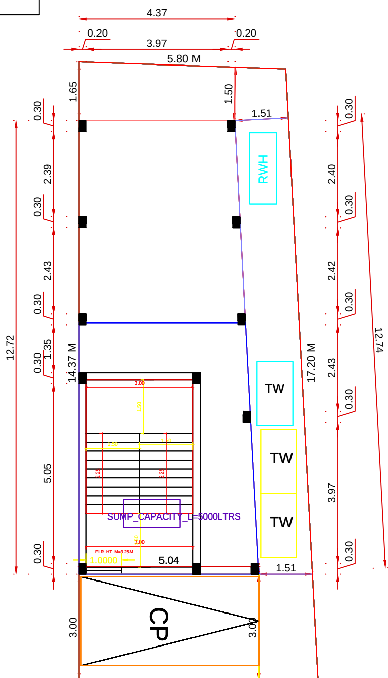
TYPICAL_FLOOR_PLAN=1,2 (PROPOSED)
