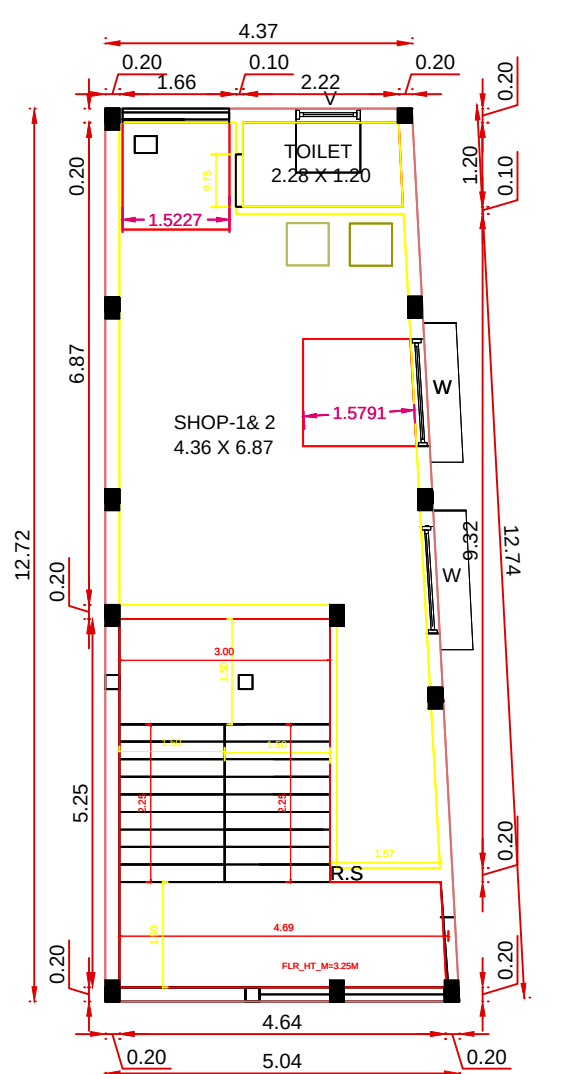
TYPICAL_FLOOR_PLAN=1,2 (PROPOSED)
